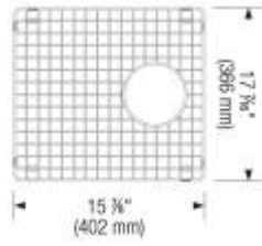
Stainless Steel Sink Grid 406398
